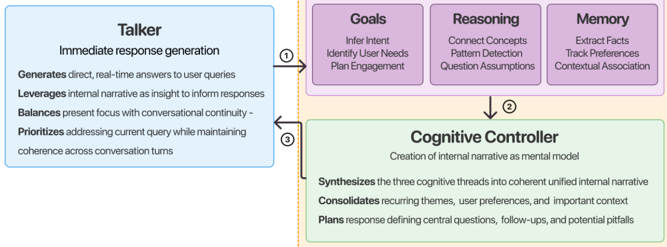
Figure 2: MIRROR component overview showing the information consolidation cycle. The Thinker (Inner Monologue Manager + Cognitive Controller) implements parallel-to-unified synthesis; the resulting narrative becomes globally available to the Talker.
